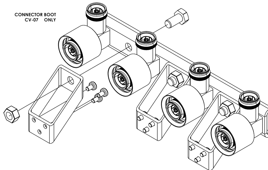
CV-07 Parts
