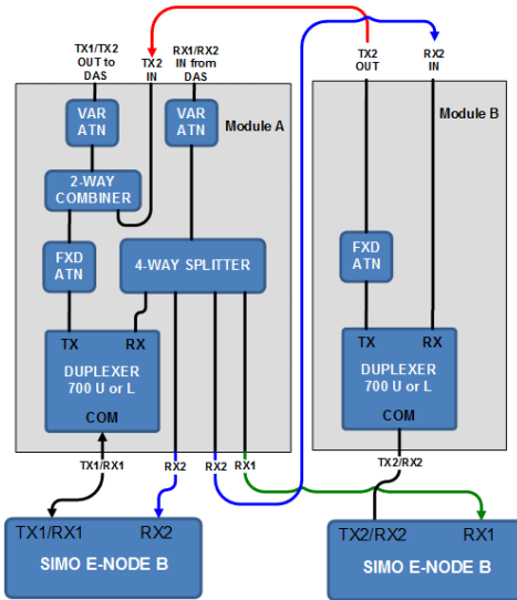
Figure IV - Shared SIMO E-Node B Configuration with SIMO Output to DAS System
