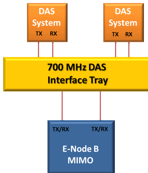
Figure II - Single MIMO E-Node B Configuration with MIMO Output to DAS System
