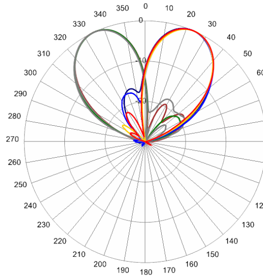
2500 MHz Azimuth
