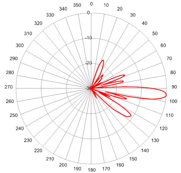
2500 MHz Elevation 5°
