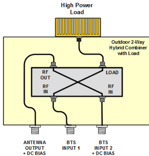
Hybrid Combiner Block Diagram
