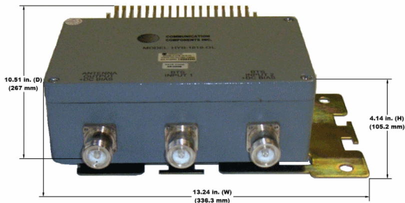
Hybrid Combiner Outline Drawing
