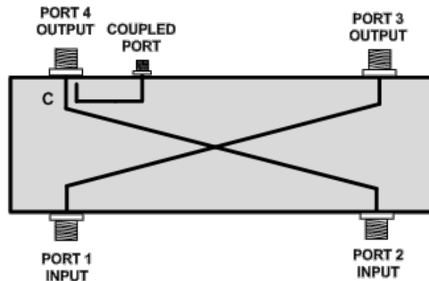
2 x 2 Hybrid Combiner Block Diagram
