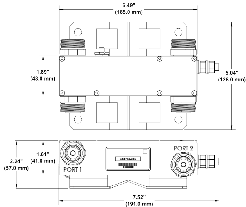
Hybrid Combiner Outline Drawing
