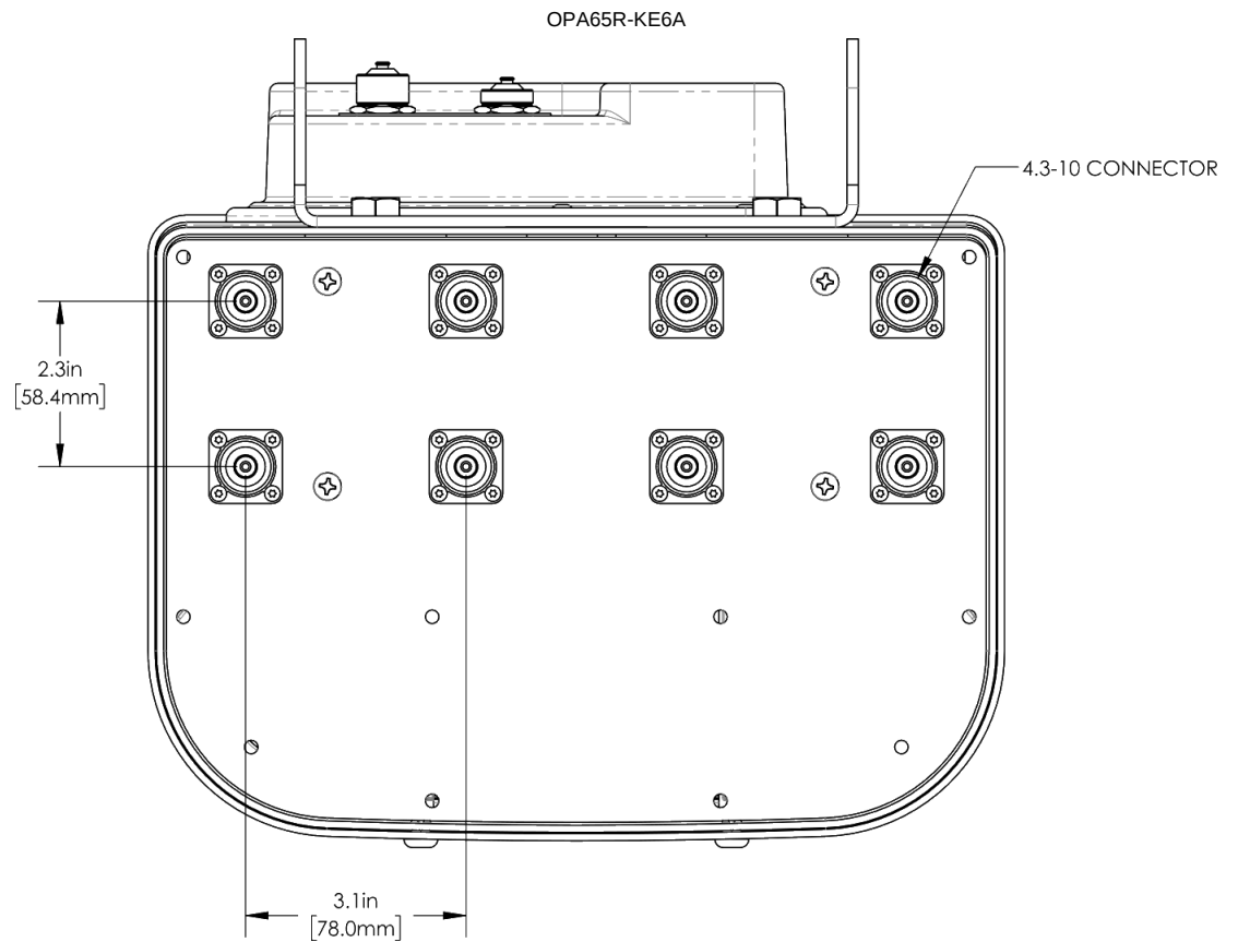
Connection Spacing Diagram
