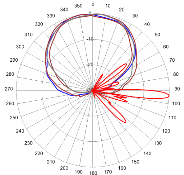
1880 MHz Azimuth with Elevation 4°
