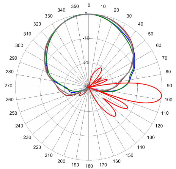
763 MHz Azimuth with Elevation 7°
