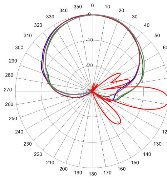
645 MHz Azimuth with Elevation 7°
