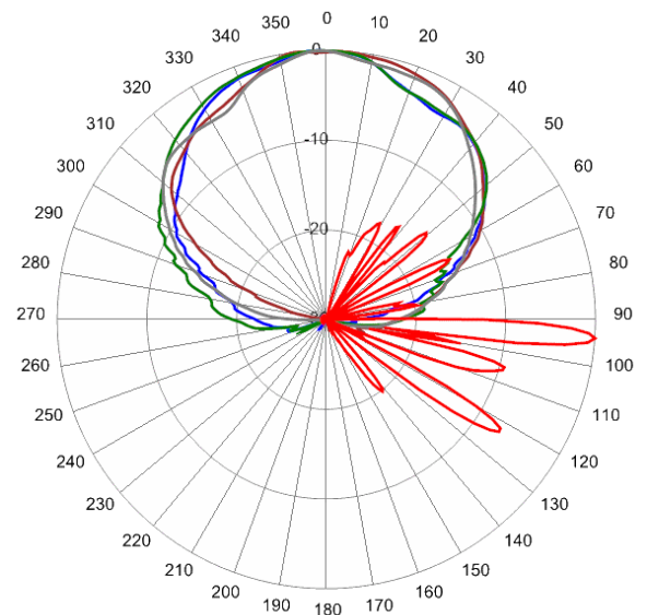
2540 MHz Azimuth with Elevation 4°
