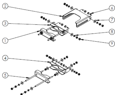
Fig. 1: Adjustable Mast Bracket BOM
