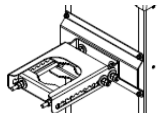
Fig. 6: Detail Of Adjustable Tilt Bracket
